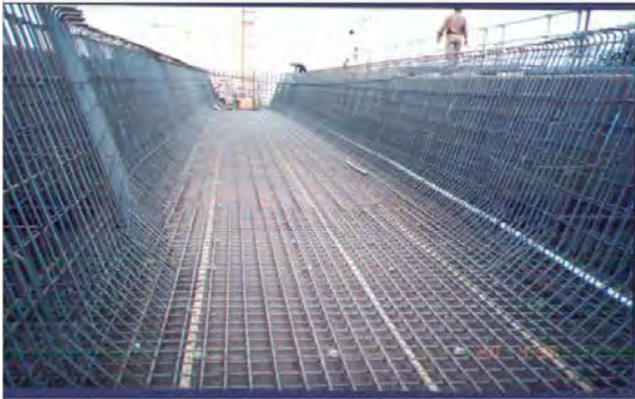
The Project Of Suez Canal Bridge Central Section In The Arab Republic Of Egypt (Kajima NKK-Nippon Consortium) Box Girder Work.
